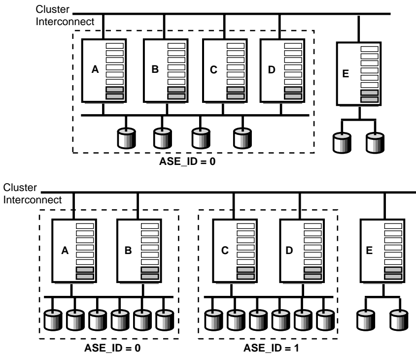
Figure 3–1: Assigning ASE_IDs to Systems in a Cluster
